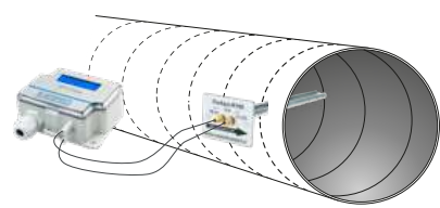
Flow Measurement in Duct
