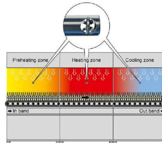
Air Velocity Sensor for Sterilization Tunnel
