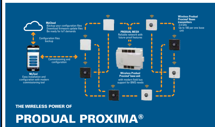
Indoor Wireless monitoring system (Temp., rH, CO 2 )
