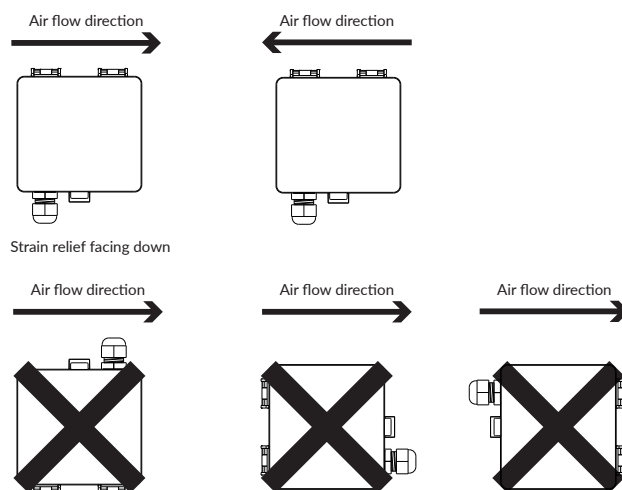
Figure 1c - Mounting orientation
