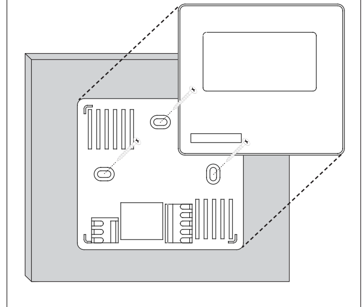
Figure 1 - Surface mounting
