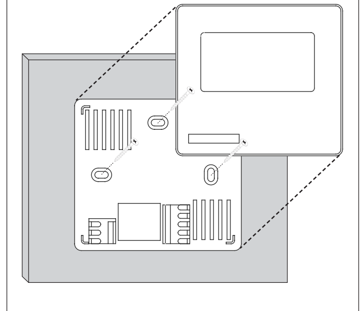
Figure 1 - Surface mounting
