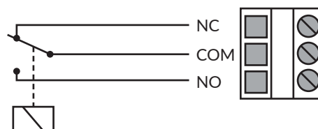
Figure 2c - Wiring diagram: Relay
