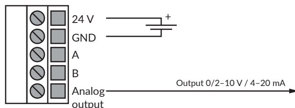
Figure 2b - Wiring diagram: Power input & signal output
